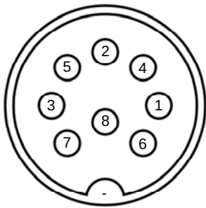
DIN 8p Male To control unit
