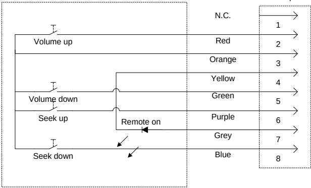
Remote Control Unit
