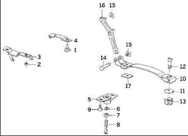
Regular Seat - Seat Mounting Hardware
