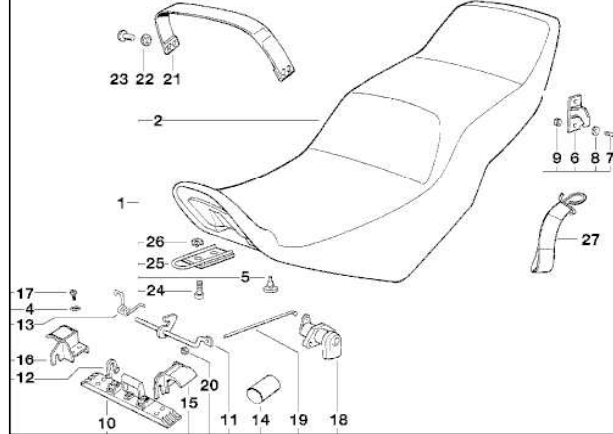
Low Seat - Seat Mounting Hardware
