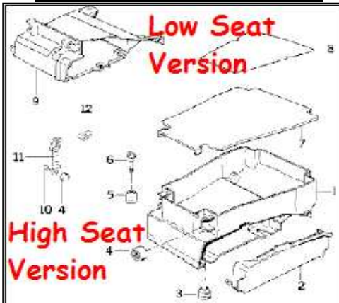
Different L-Jetronic Holder Under The Seat
